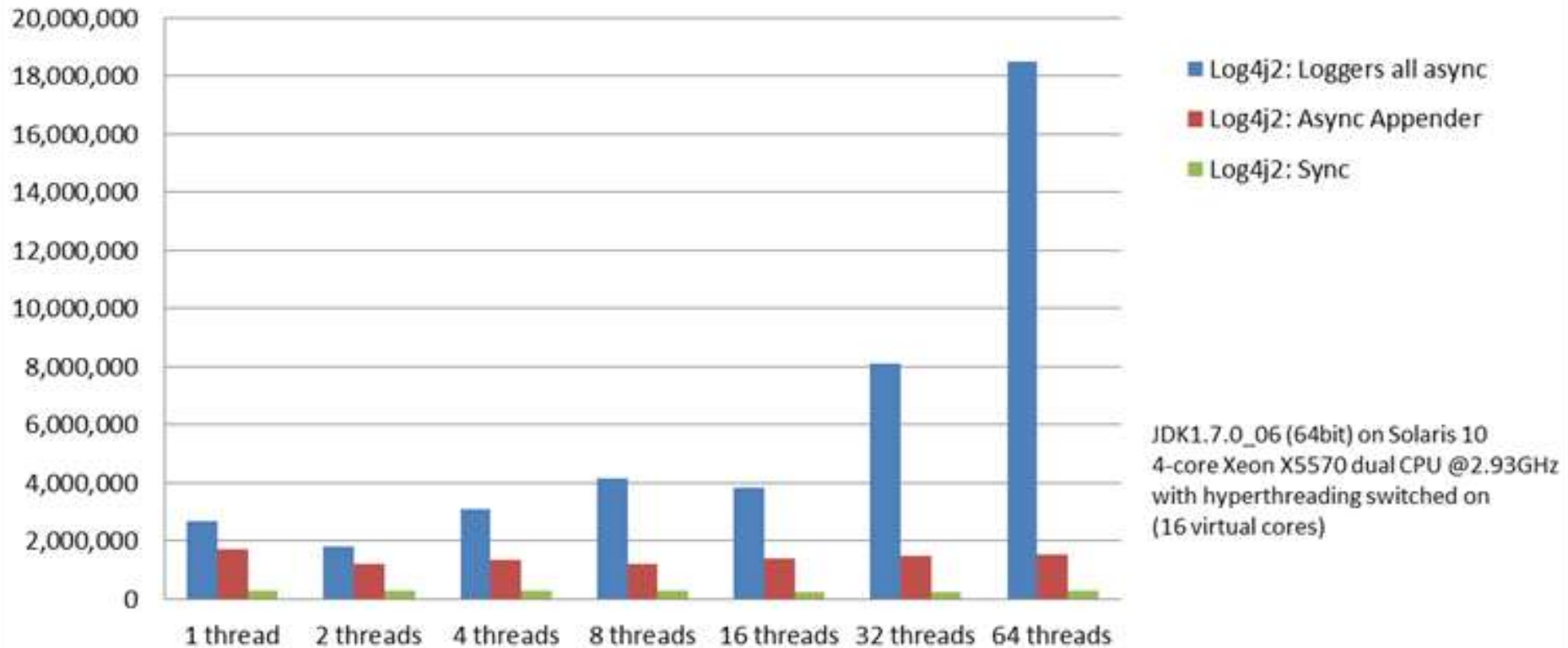
Sync vs Async Logging Throughput (msg/sec) - higher is better
